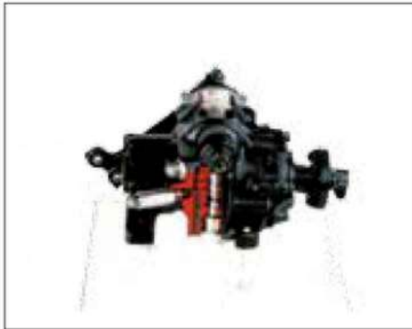
■ Recirculating ball and nut steering anatomical model
